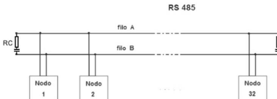
Fig. 2 AC termination
